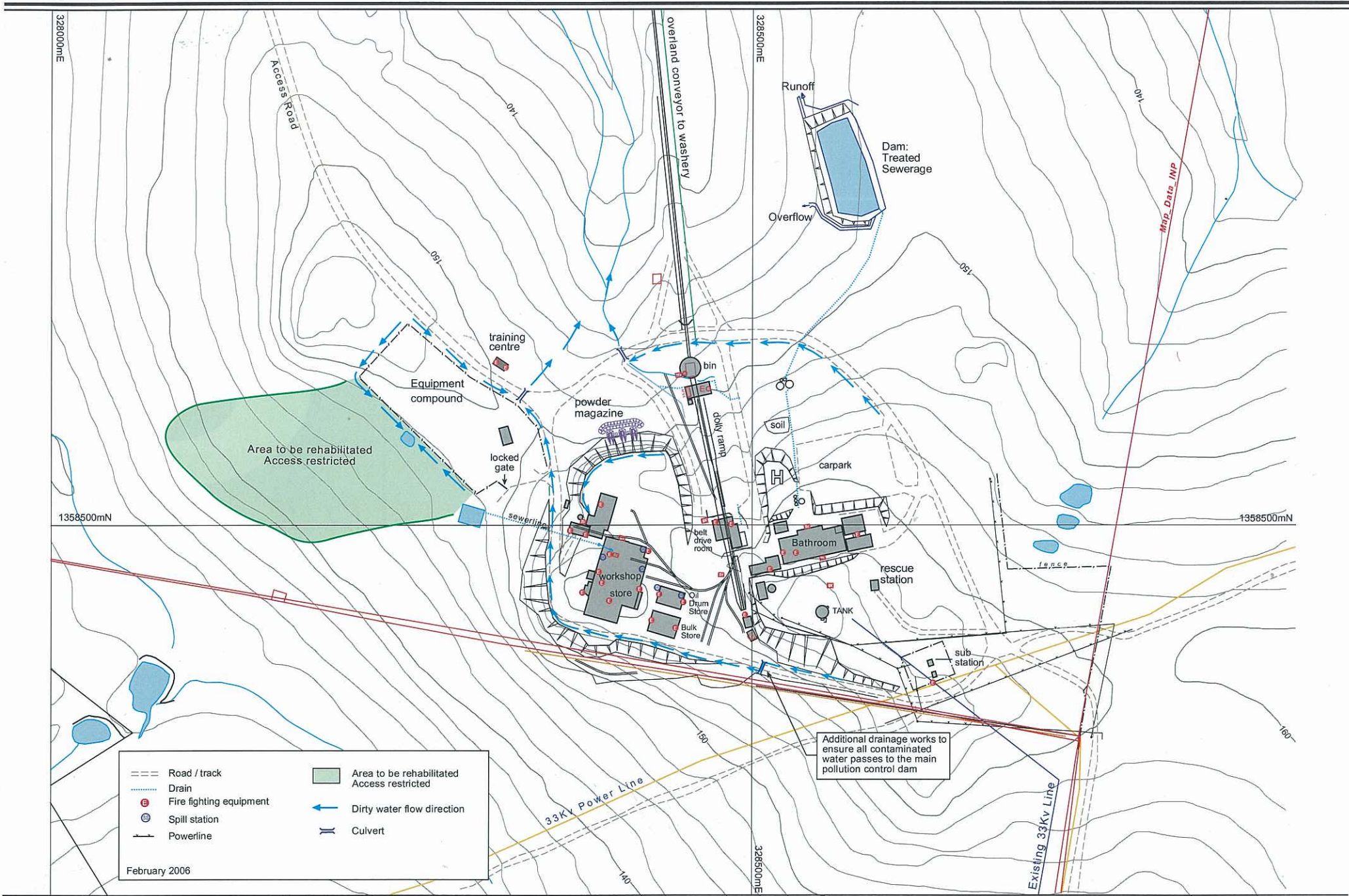
FIGURE 11 Austar Coal Mine - Surface Facilities
