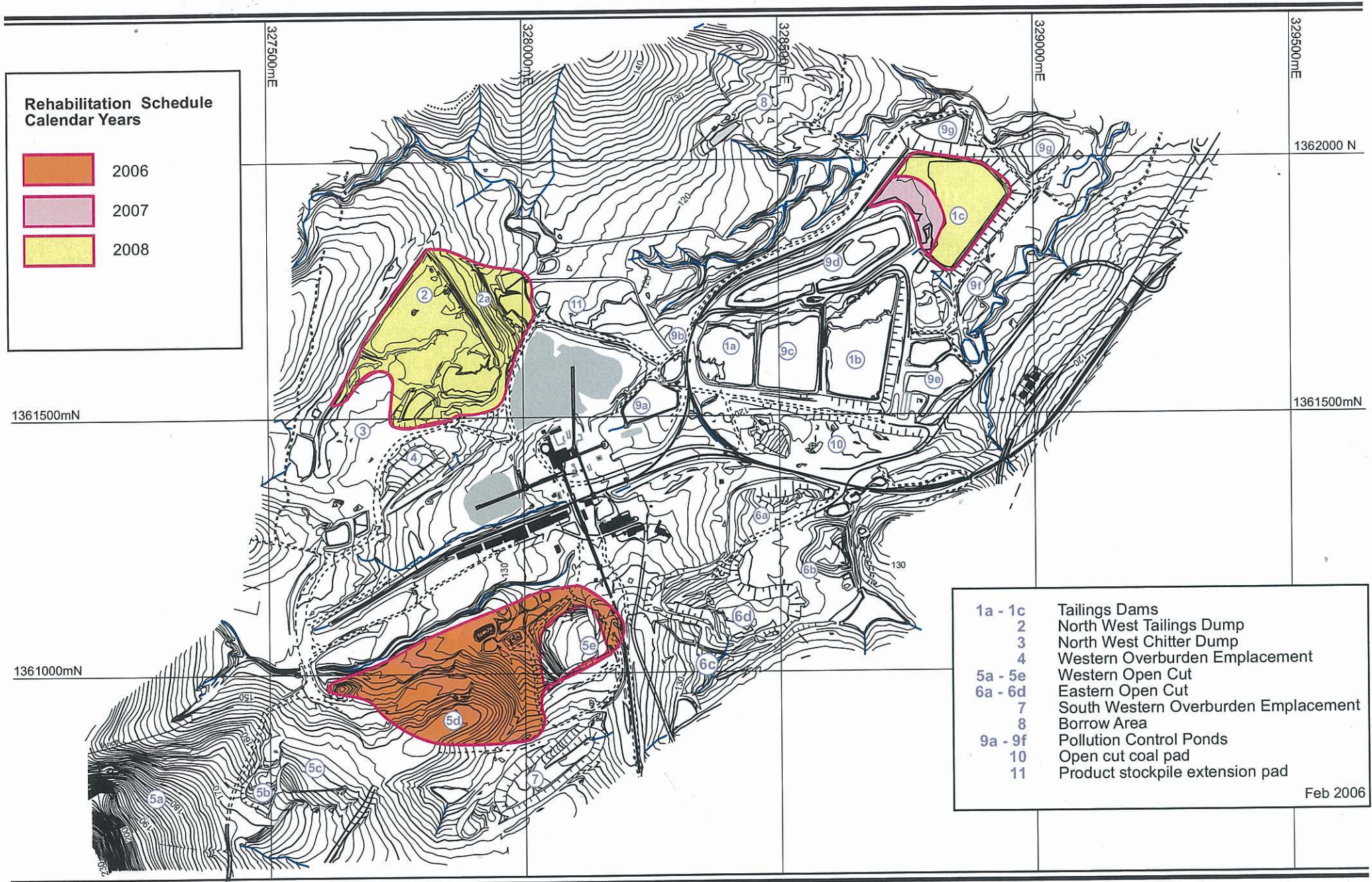
FIGURE 12 Austar Washery - Rehabilitation Schedule
