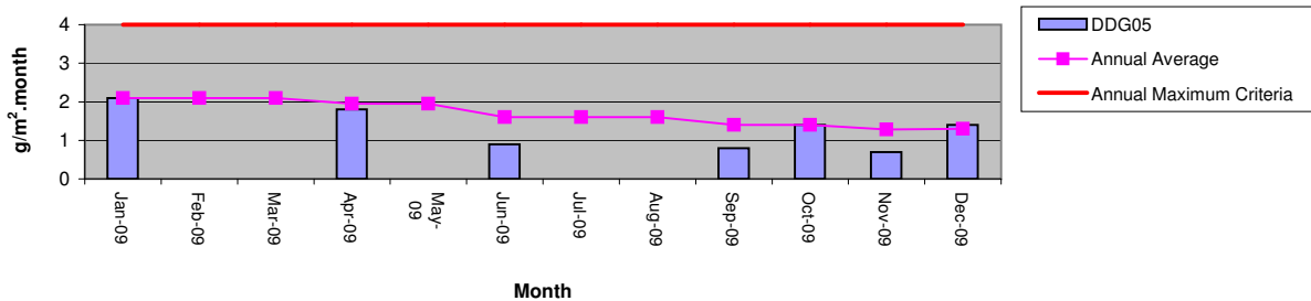
Austar Dust Gauge DDG05 - Insoluble Solids
