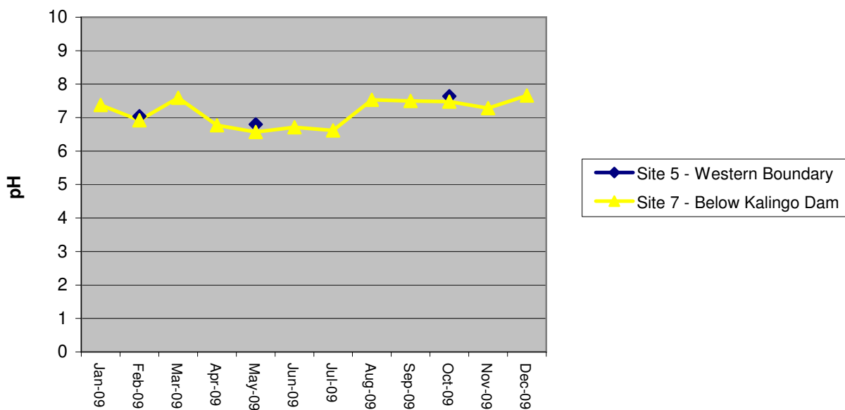
Surface Water Sites 5 and 7 pH - 2009
