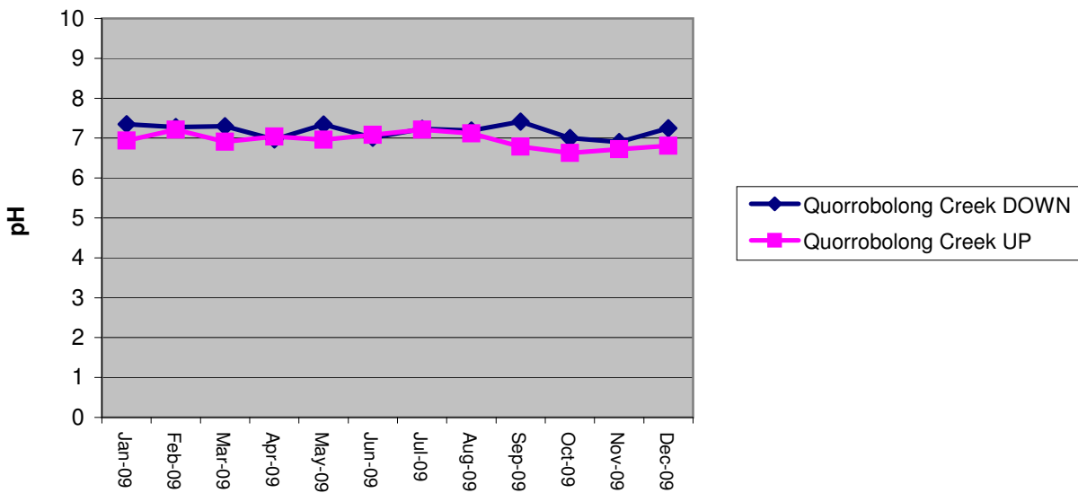
Surface Water Sites Quorrobolong Creek Up and Down pH - 2009
