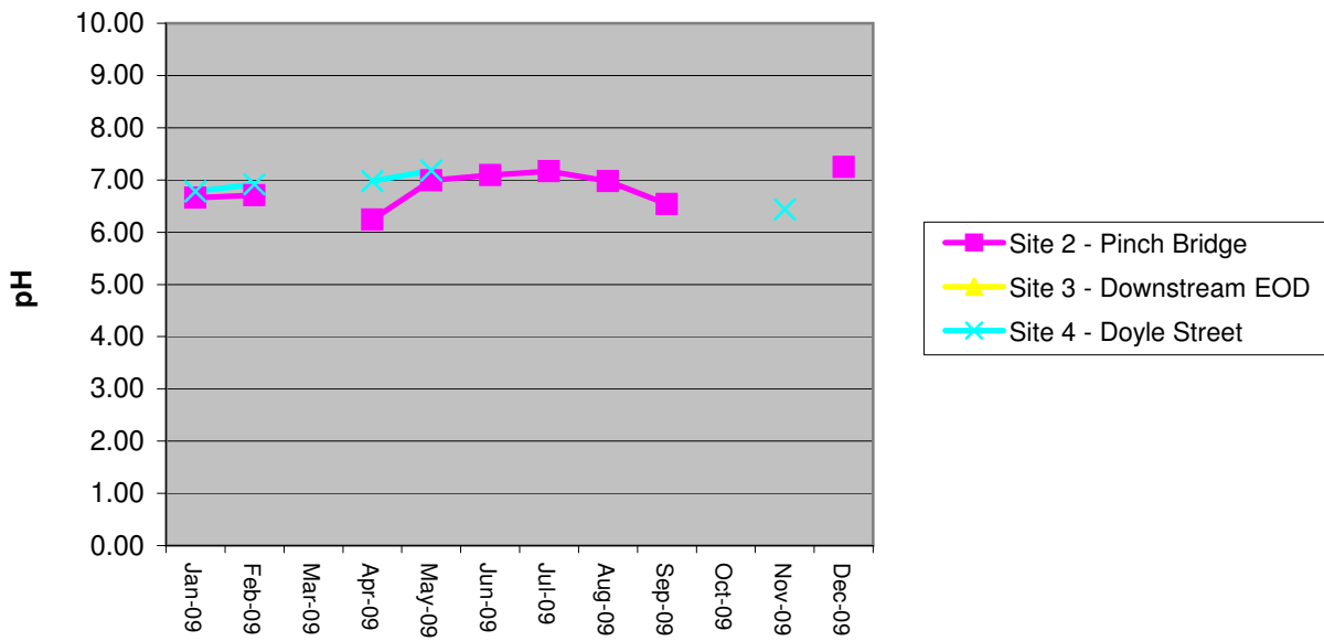
Surface Water Sites 2,3 and 4 pH - 2009
