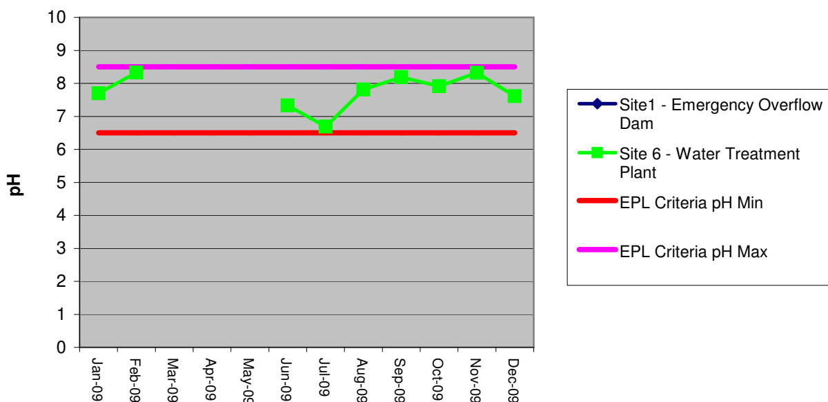
Surface Water Sites 1 and 6 pH - 2009
